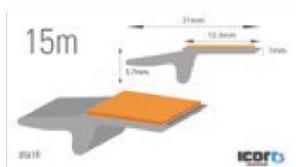
VW GOLF III 91-97 HOTL SEMI-ENCAPS PROFILE 15M ROL 8541R COP: A
